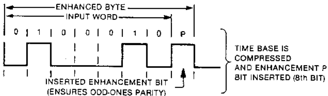
Figure 7-5.—Enhanced non-return-to-zero-level (E-NRZ-L) digital encoding method.
